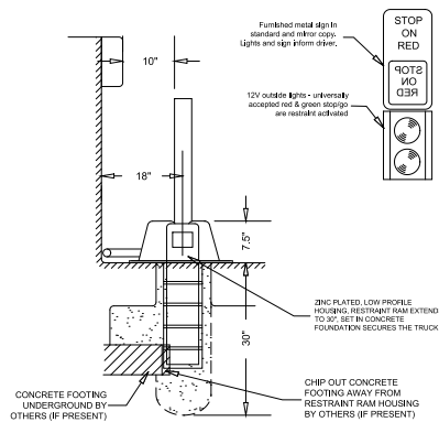
SECTION @ RESTRAINT
