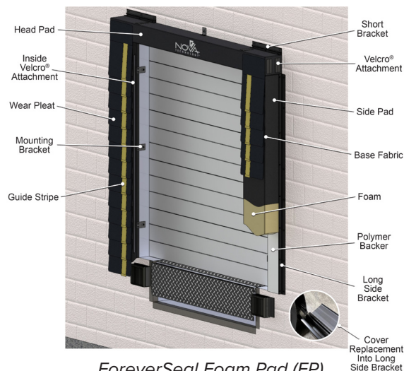
ForeverSeal Foam Pad (FP) Series Dock Seal
