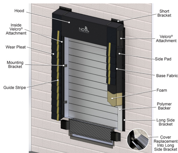
ForeverSeal Foam Pad Hood (FPH) Dock Seal
