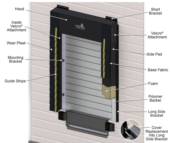
ForeverSeal Foam Pad Hood (FPH) Dock Seal
